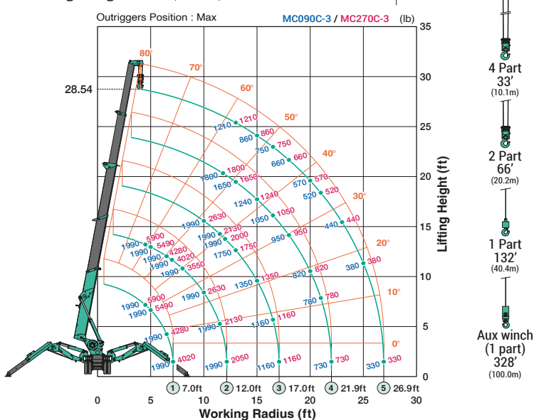
Working Range Chart (4Part)
